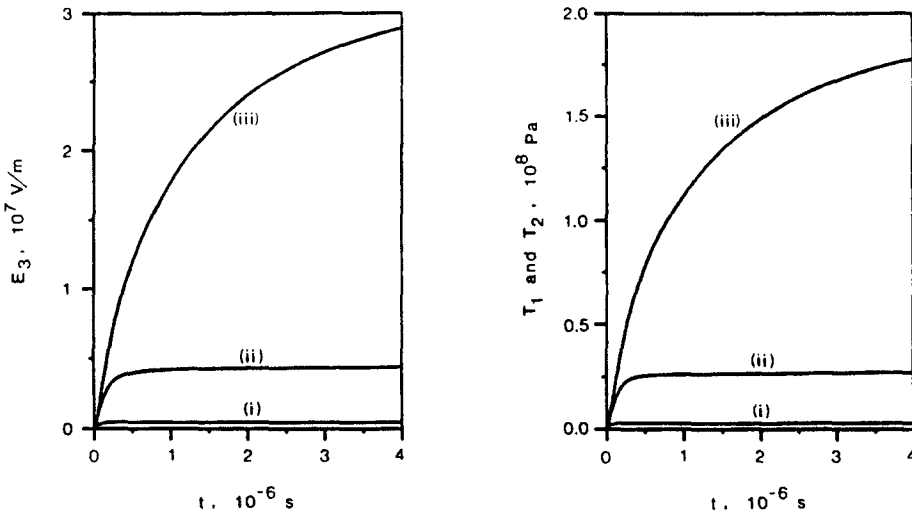
Fig. 7. Electric field component E_3 and stress components T_1 and T_2 ahead of the shock as functions of time: (i) 10^3 \Omega , (ii) 10^4 \Omega , and (iii) 10^5 \Omega . These results correspond to intermediate depoling rate.
