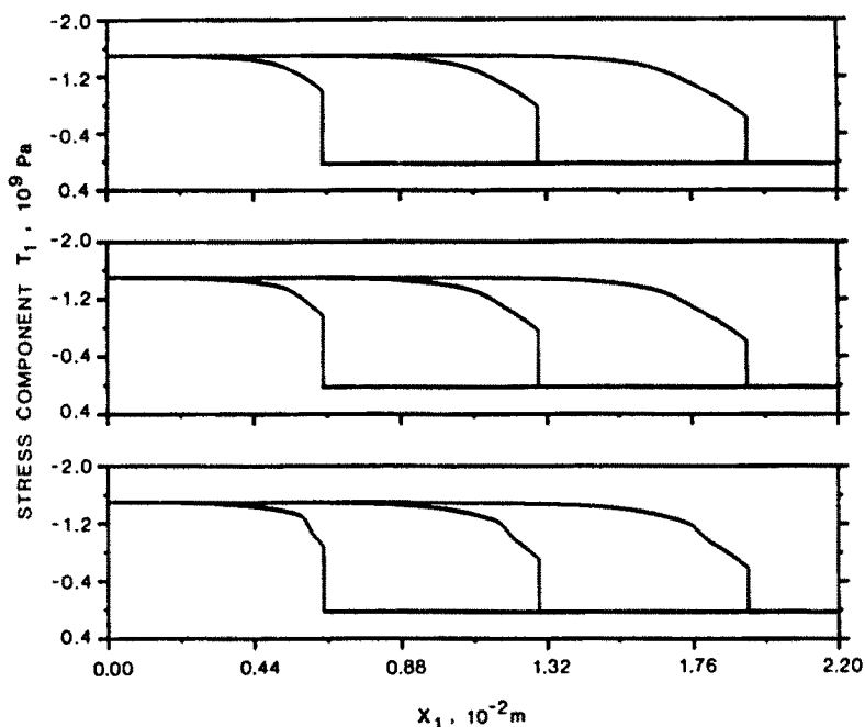
Fig. 4. Stress component T_1 as function of position at three different times. Top curves correspond to slowest depoling rate, middle curves correspond to intermediate depoling rate, and bottom curves correspond to fastest depoling rate. The resistance of the external circuit is 10^6 \Omega .
