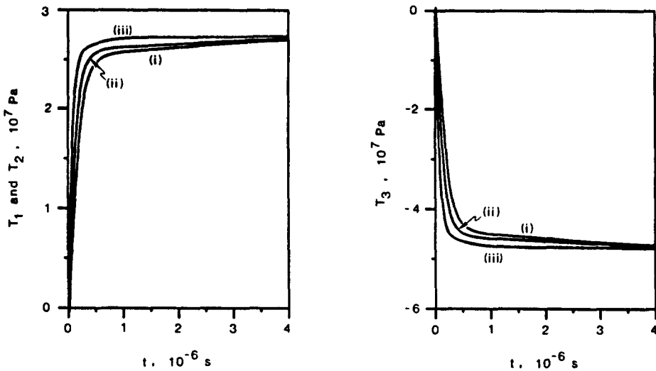
Fig. 6. Stress components T_1 , T_2 and T_3 ahead of the shock as functions of time: (i) slowest depoling rate, (ii) intermediate depoling rate, and (iii) fastest depoling rate. The resistance of the external circuit is 10^4 \Omega .
